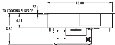
COMPACT GRIDDLE MODULE
