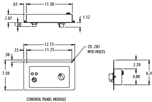
CONTROL PANEL MODULE
