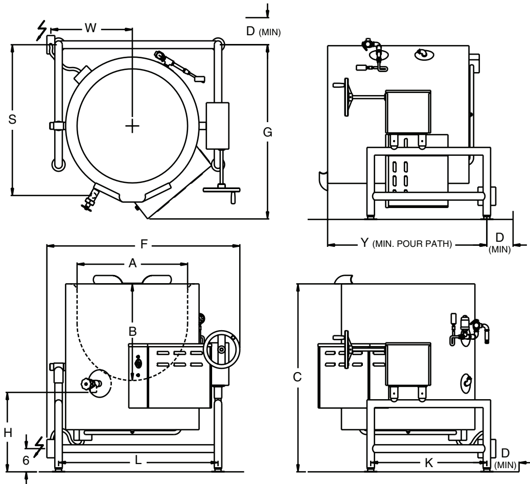
DRAWING REPRESENTS 60 GALLON MODEL WITH OPTIONAL 1 1/2" DRAW-OFF
