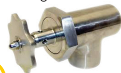
2" Tangent draw-off
