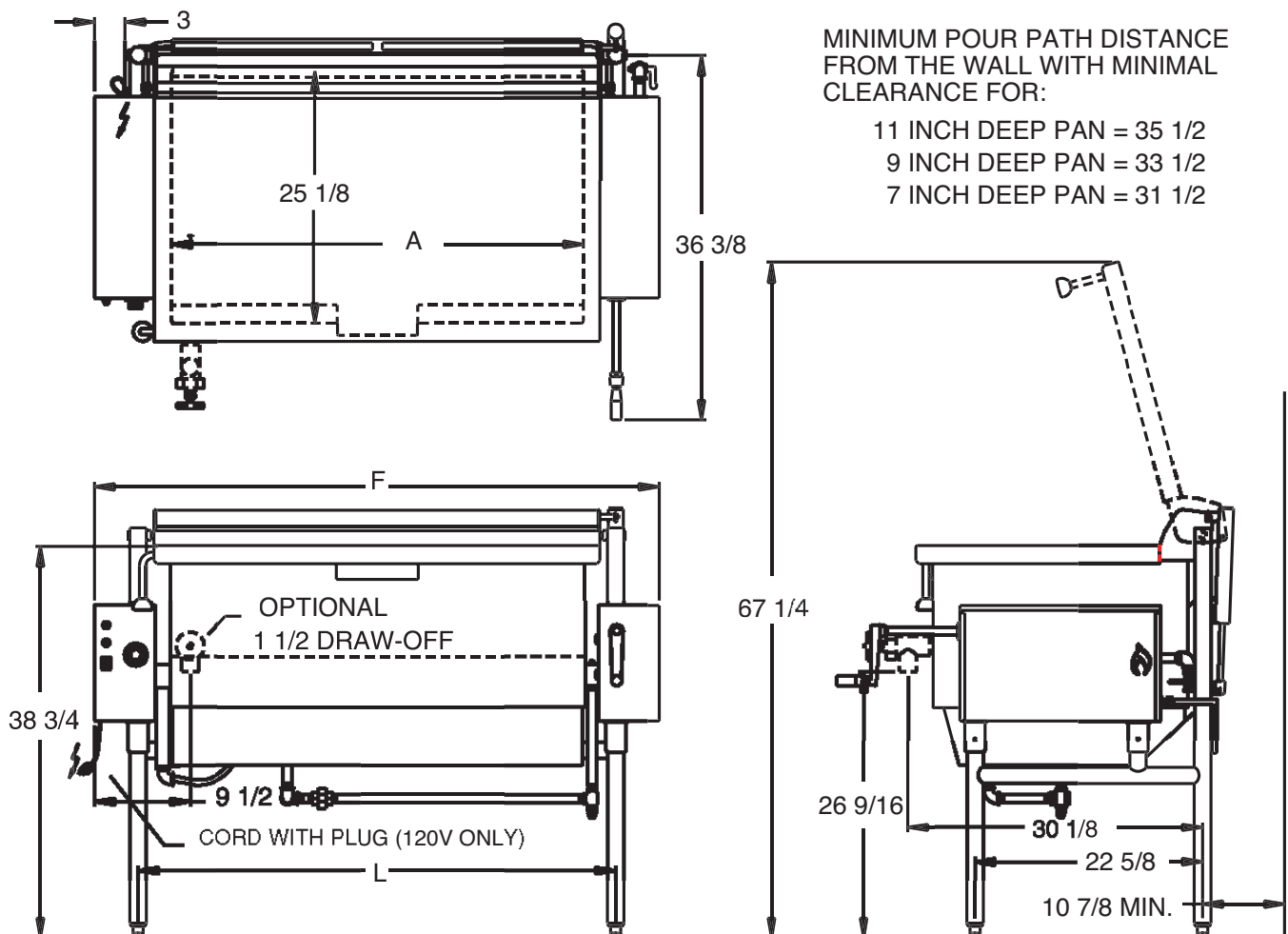
Drawing Represents Model ALGTSE-40 with optional 1.5" draw-off
